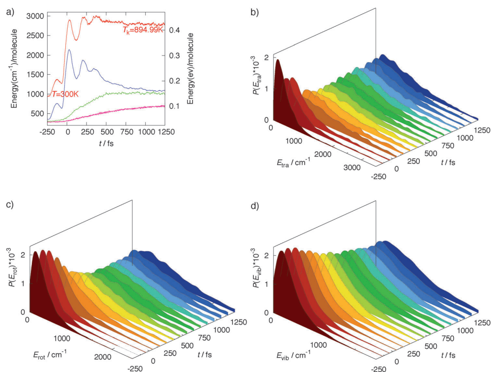
Figure 1. a) Average kinetic energy of each monomer partitioned according to; red: total kinetic energy, blue: translational kinetic energy, green: rotational kinetic energy, and pink: vibrational kinetic energy. T_k and T refer to kinetic and equilibrium temperatures, respectively. Probability distributions per water molecule of translational (b), rotational (c), and vibrational (d) energies for different time delays. These are Maxwell–Boltzmann distributions for t = -250 fs (see the Supporting Information) and are normalized at all times \int_0^\infty P(E) dE = 1 .
